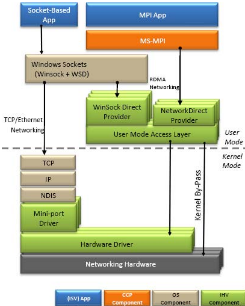
Figure 8. Networking architecture
